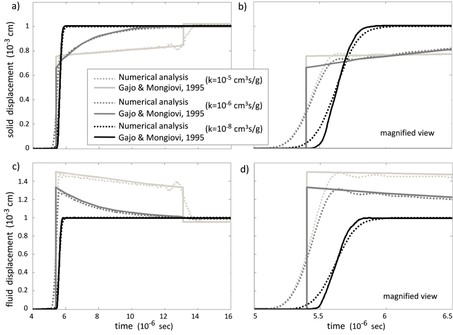
Figure 7: Comparison between numerical analysis and analytical solution by Gajo and Mongiovi (1995) for three different values of viscous coupling, k : a) solid displacement versus time from 4\text{--}16 \times 10^{-6} sec, b) solid displacement versus time from 5\text{--}6.5 \times 10^{-6} sec, c) fluid displacement versus time from 4\text{--}16 \times 10^{-6} sec, and d) fluid displacement versus time from 5\text{--}6.5 \times 10^{-6} sec, obtained 1 cm below the surface.
