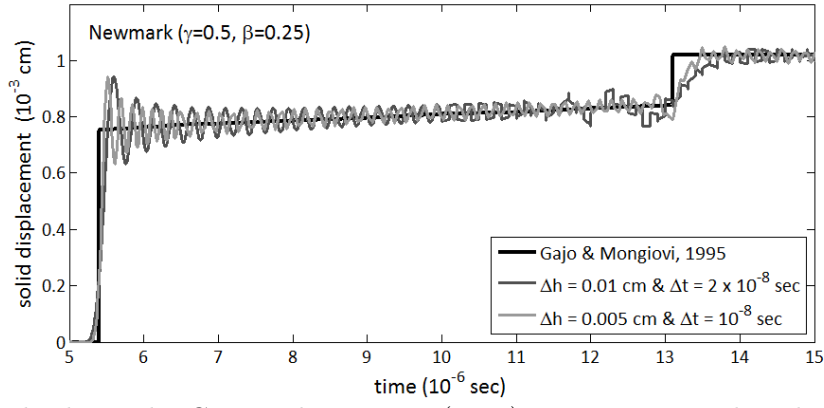
Figure 8: Analytical solution by Gajo and Mongiovi (1995) versus numerical analysis with no numerical damping ( \gamma = 0.5 and \beta = 0.25 ) for two different combinations of spatial and temporal discretization: i) \Delta h = 0.01 cm and \Delta t = 2 \times 10^{-8} sec, ii) \Delta h = 0.005 cm and \Delta t = 10^{-8} sec, in the case of viscous coupling k = 10^{-5} cm 3 s/g.
