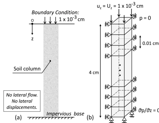
Figure 6: a) A representative soil column subjected to a step vertical displacement equal to 1.0 \times 10^{-3} cm at the surface, and b) the finite element mesh and the applied boundary conditions used for numerical modeling.
