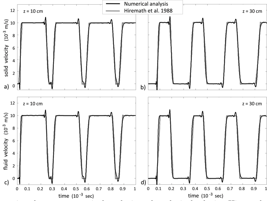
Figure 16: Comparison between numerical analysis and analytical solution Hiremath et al. (1988) for the case of strong viscous coupling ( k = 0.148 \times 10^{-8} \text{ cm}^3\text{s/g} ) in terms of time histories of: a) solid velocity at 10 cm below the surface, b) solid velocity at 30 cm below the surface, c) fluid velocity at 10 cm below the surface and, d) fluid velocity at 30cm below the surface.
