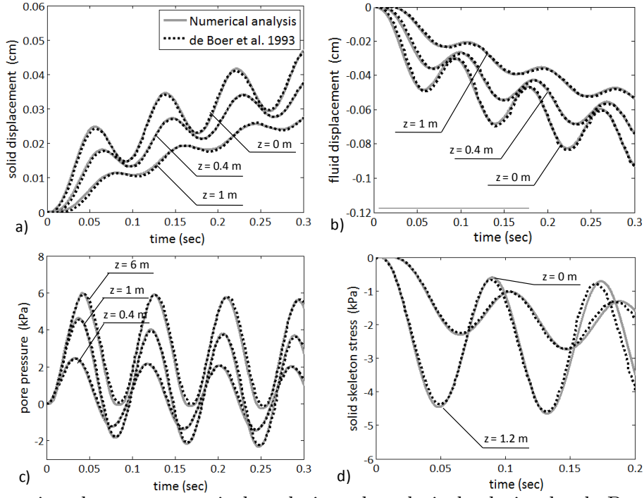
Figure 15: Comparison between numerical analysis and analytical solution by de Boer et al. (1993) in terms of a) solid displacements, b) fluid displacements, c) pore pressure and d) solid skeleton stress versus time for different depths.
