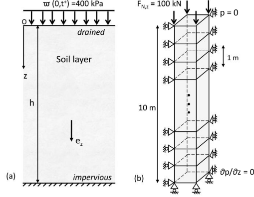
Figure 2: (a) The geometry of the soil layer of thickness h under uniform constant vertical pressure \varpi = 400 kPa applied at the surface, and (b) the finite element mesh with the appropriate boundary conditions and loading at top.
