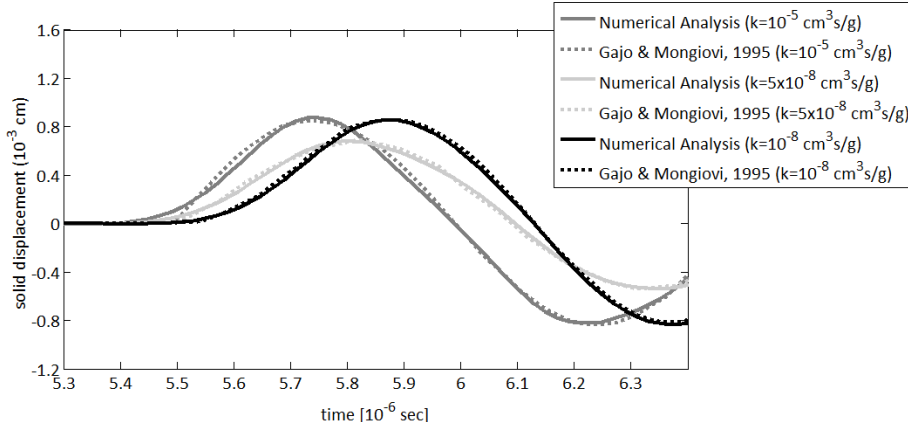
Figure 11: Comparison between numerical analysis and analytical solution by Gajo and Mongiovi (1995) in terms of solid displacement, obtained 1 m below the surface, for three different values of viscous coupling, k .
