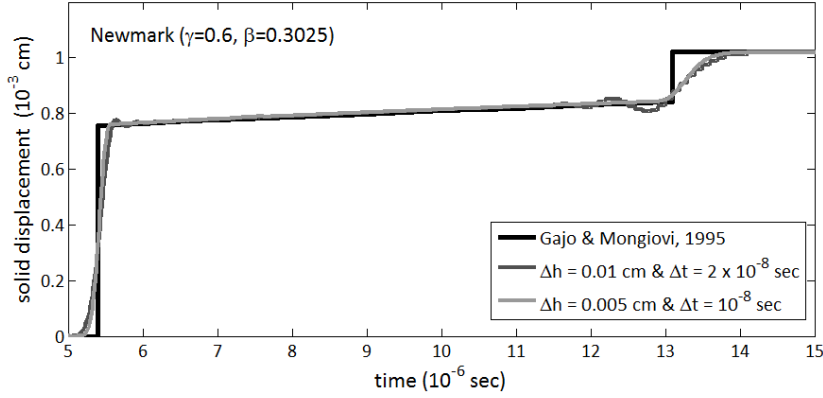
Figure 9: Analytical solution by Gajo and Mongiovi (1995) versus numerical analysis with no numerical damping ( \gamma = 0.6 and \beta = 0.3025 ) for two different combinations of spatial and temporal discretization: i) \Delta h = 0.01 cm and \Delta t = 2 \times 10^{-8} sec, ii) \Delta h = 0.005 cm and \Delta t = 10^{-8} sec, in the case of viscous coupling k = 10^{-5} cm 3 s/g.
