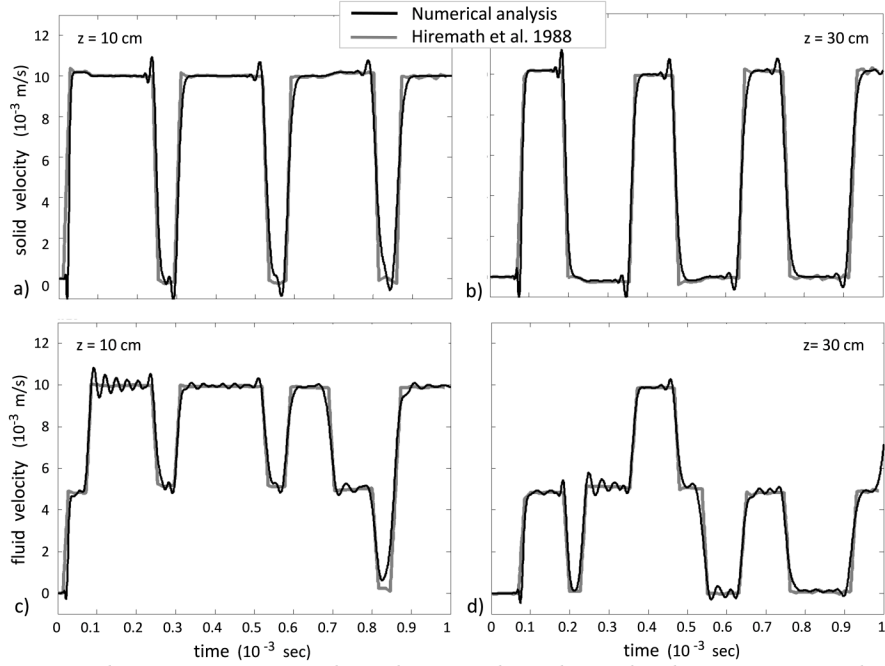
Figure 17: Comparison between numerical analysis and analytical solution Hiremath et al. (1988) for the case of weak viscous coupling ( k = 0.148 \times 10^{-2} \text{ cm}^3\text{s/g} ): a) solid velocity at 10 cm below the surface, b) solid velocity at 30 cm below the surface, c) fluid velocity at 10 cm below the surface and d) fluid velocity at 30cm below the surface, versus time.
