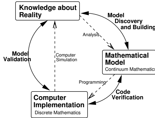
Figure 1: Schematic representation of the role of Verification and Validation on numerical modeling (inspired from Oberkampf et al. (2002); Roy and Oberkampf (2011) and Oden et al. (2010a)).
