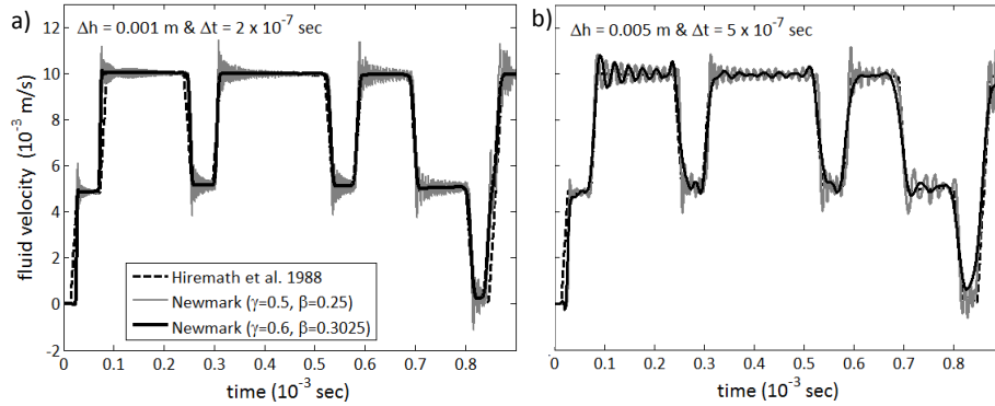
Figure 19: Analytical solution Hiremath et al. (1988) versus numerical analysis with no numerical damping ( \gamma = 0.6 and \beta = 0.3025 ), in terms of fluid velocity time history at 10 cm below the surface, for the case of weak viscous coupling ( k = 0.148 \times 10^{-2} \text{ cm}^3\text{s/g} ): a) \Delta h = 0.001 \text{ m} and \Delta t = 2 \times 10^{-7} \text{ sec} and b) \Delta h = 0.005 \text{ m} and \Delta t = 5 \times 10^{-7} \text{ sec} .
