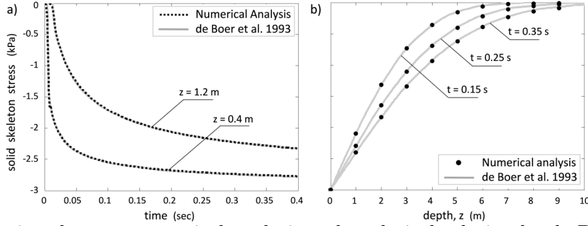
Figure 13: Comparison between numerical analysis and analytical solution by de Boer et al. (1993) in terms of a) solid-skeleton stress versus time at different depths, and b) solid-skeleton stress versus depth at different times.
