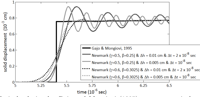
Figure 10: Analytical solution by Gajo and Mongiovi (1995) versus numerical analysis for two cases of numerical damping: a) \gamma = 0.5 and \beta = 0.25 (no numerical damping) and b) \gamma = 0.6 and \beta = 0.3025 and for two different combinations of spatial and temporal discretization: i) \Delta h = 0.01 cm and \Delta t = 2 \times 10^{-8} sec, ii) \Delta h = 0.005 cm and \Delta t = 10^{-8} sec, in case of viscous coupling k = 10^{-5} cm 3 s/g. Magnified view of the first wavefront.
