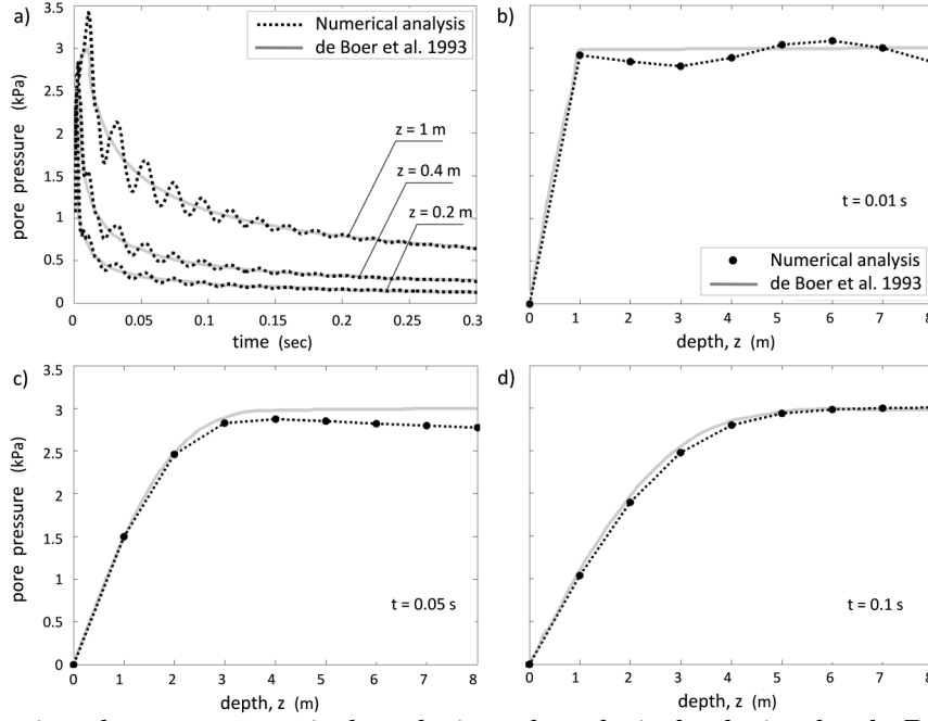
Figure 14: Comparison between numerical analysis and analytical solution by de Boer et al. (1993): a) pore fluid pressure versus time at different depths, b) pore fluid pressure stress versus depth at time t = 0.01 sec, c) pore fluid pressure stress versus depth at time t = 0.05 sec, and d) pore fluid pressure stress versus depth at time t = 0.1 sec.
