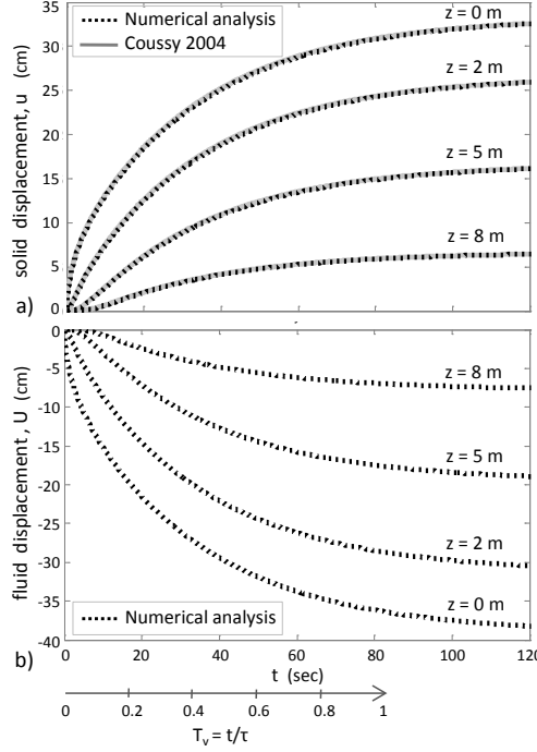
Figure 4: (a) Comparison between numerical analysis and analytical solution by Coussy (2004) in terms of time histories: a) solid-skeleton displacements, and b) fluid displacements, for various depths.
