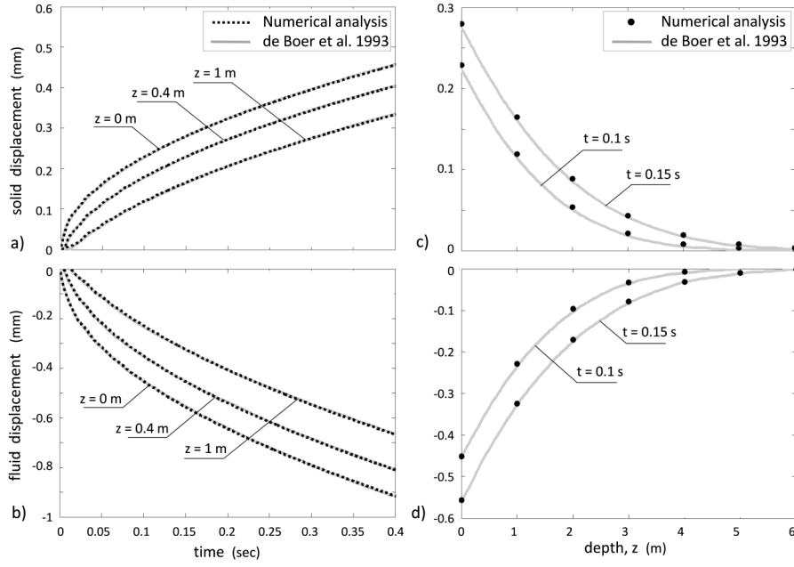
Figure 12: Comparison between numerical analysis and analytical solution by de Boer et al. (1993) in terms of a) solid displacements versus time at different depths, b) fluid displacements versus time at different depths, c) solid displacements versus depth at different times, and d) fluid displacements versus depth at different times.
