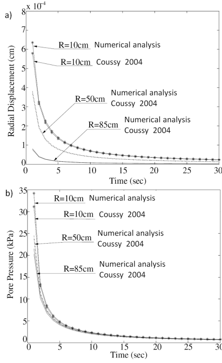
Figure 5: Comparison between numerical analysis and analytical solution by Coussy (2004): a) radial displacement, and b) pore pressure versus time at different distances, R , from the center of the model.
