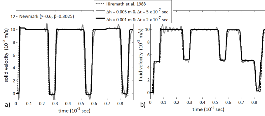
Figure 18: Analytical solution Hiremath et al. (1988) versus numerical analysis, with two different combinations of spatial and temporal discretization and numerical damping ( \gamma = 0.6 and \beta = 0.3025 ), for the case of weak viscous coupling ( k = 0.148 \times 10^{-2} \text{ cm}^3\text{s/g} ): a) solid velocity at 10 cm below the surface and b) fluid velocity at 10 cm below the surface, with time.
