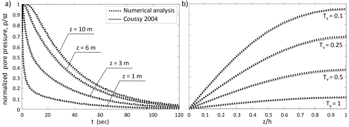
Figure 3: Comparison between numerical analysis and analytical solution by Coussy (2004): a) normalized pore pressure at various depths with respect to real time, t , and b) distribution of normalized pore pressure with normalized depth, z/h , for different time factors, T_v .
